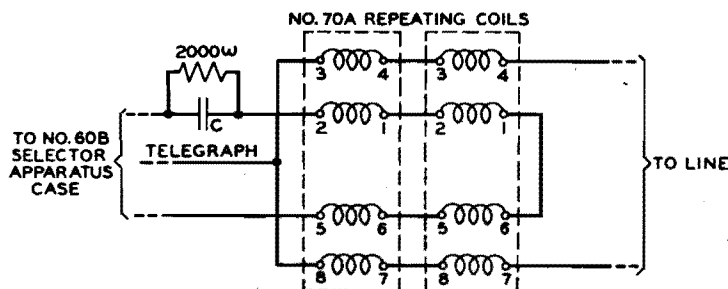
Figure 23—Selector Circuit Operated Through Two No. 70A Repeating Coils in Series Aiding
