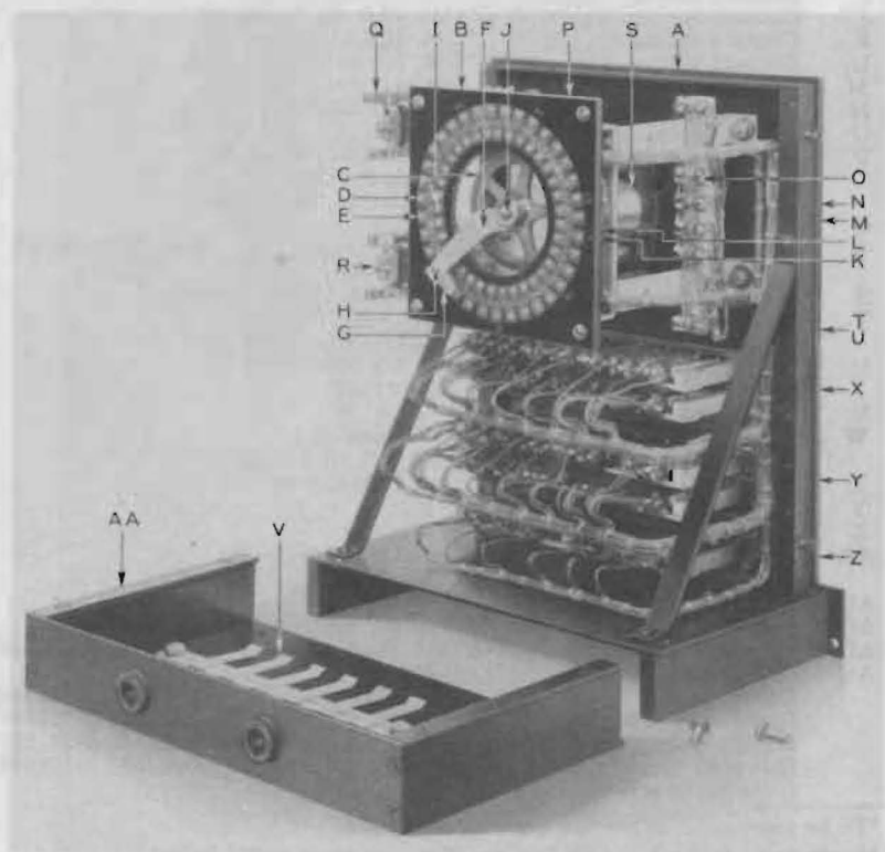
Figure 45—No. 62 Type Selector Key
