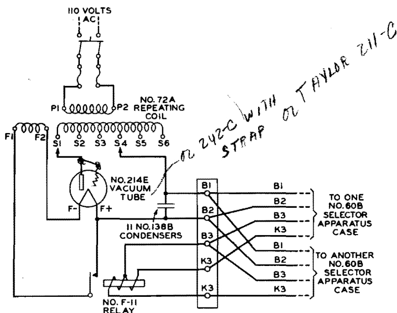
Figure 5—Schematic Circuit of No. 60B Vacuum Tube Rectifier
