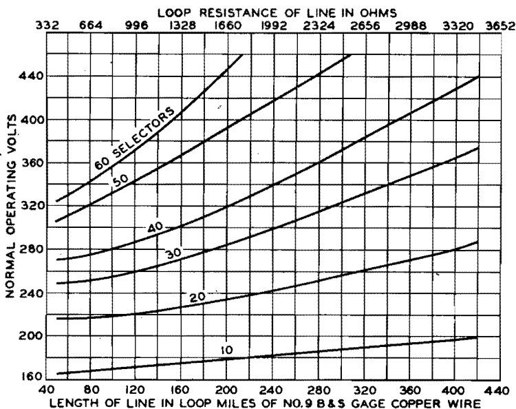
Figure 25—Curves for No. 160 Type Selector Sets Operated Through No. 341A Transformer
