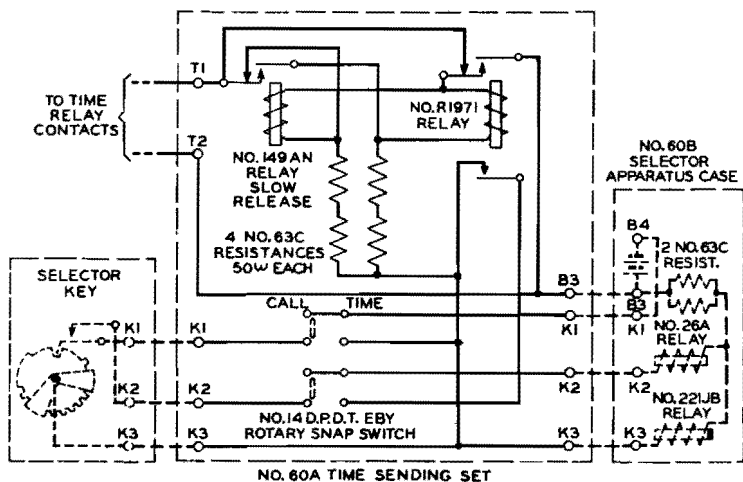
Figure 20—Schematic Circuit of No. 60A Time Sending Set
