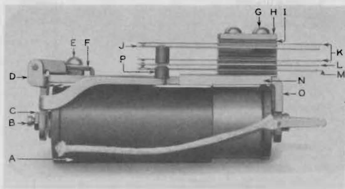
Figure 41—No. 221JB Relay
