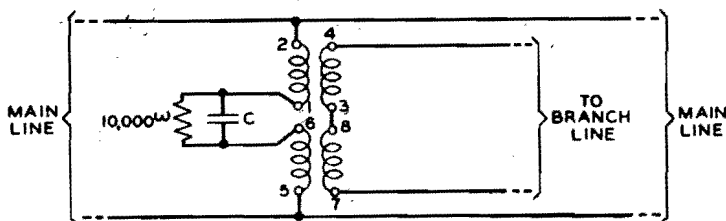
Figure 29—Branch Line Operated Through a Transformer
