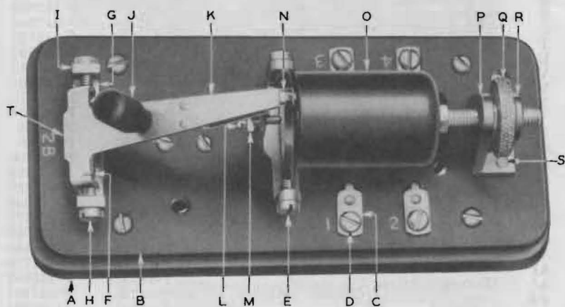
Figure 40—No. 2B Circuit Breaker
