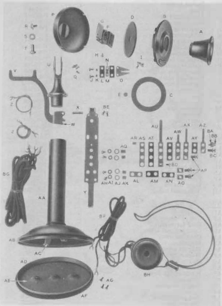
Figure 49—No. 1142AB Desk Stand
