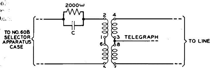
Figure 22—Selector Circuit Operated Through No. 341A Transformer
