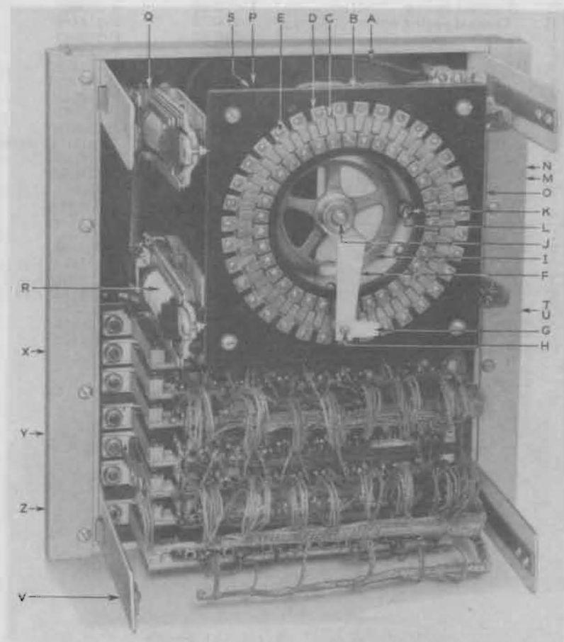
Figure 46—No. 63 Type Selector Key
