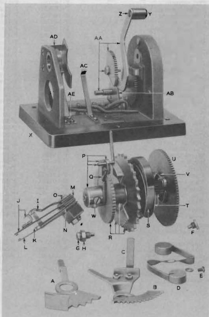
Figure 44—No. 61 Type Selector Key
