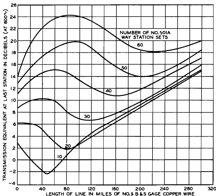
Figure 35—Curves of Transmission Equivalent at Last Way Station for Different Length of Lines and Number of Stations
