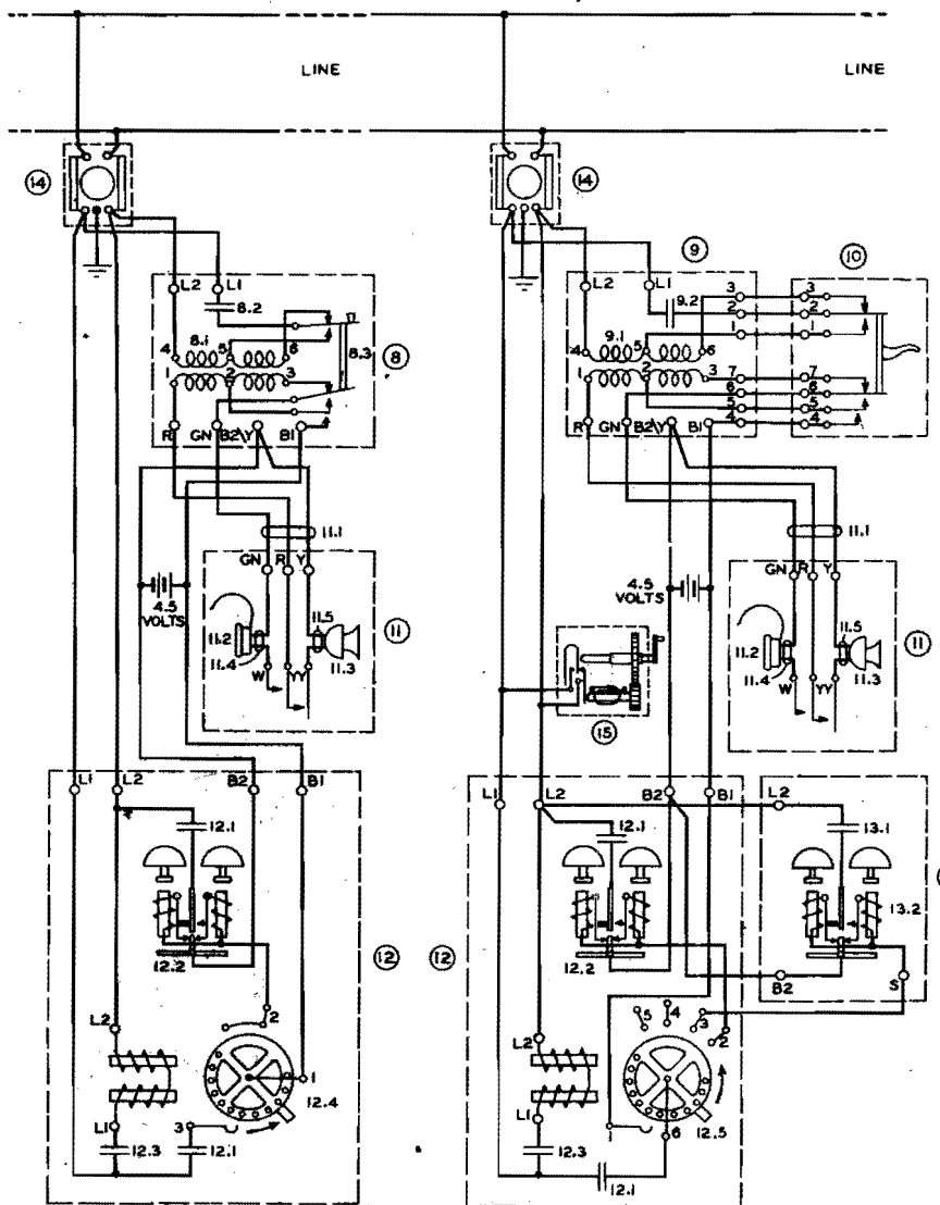
Figure 32—Schematic Circuit of Way Station-Telephone and Selector Equipment
