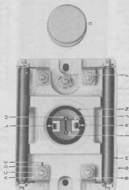
Figure 51—No. 98B Protector
