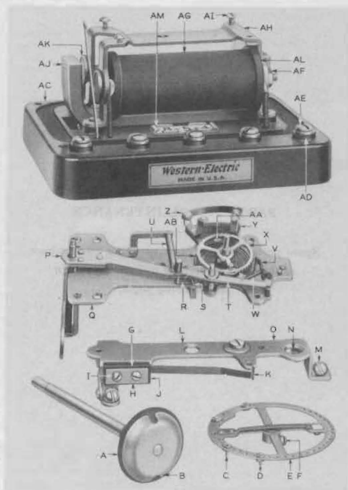
Figure 39—No. 60 Type Selector
