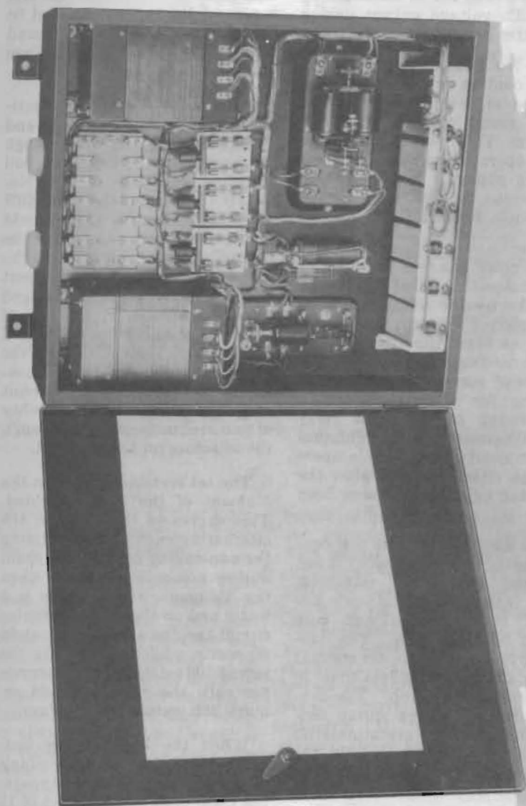
Figure 6—No. 60B Selector Apparatus Case (Open)
