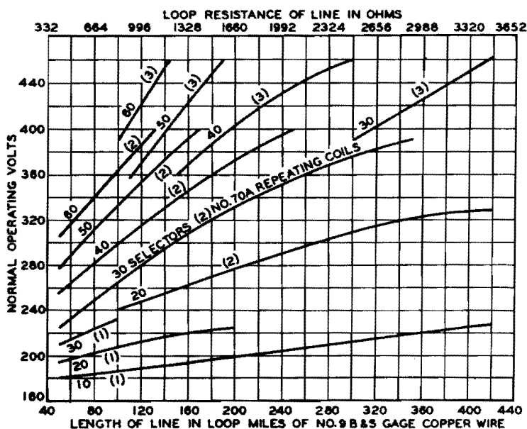
Figure 26—Curves for No. 160 Type Selector Sets Operated Through No. 70A Repeating Coils
