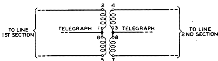
Figure 27—Intermediate Simplex Telegraph Drop
