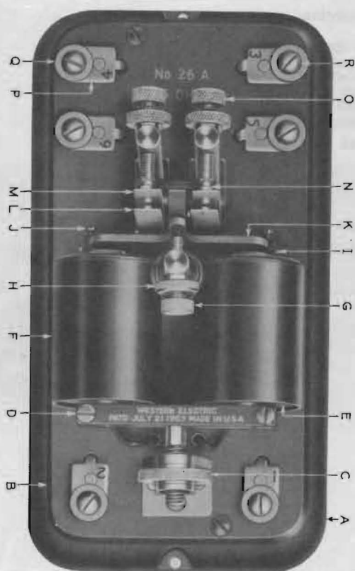
Figure 42—No. 26A Telegraph Relay
