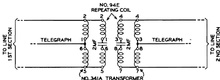
Figure 28—Intermediate Simplex Telegraph Drop with Voice Frequency By-Pass Repeating Coil
