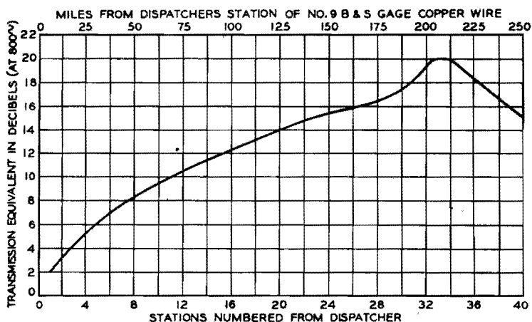
Figure 34—Curve of Transmission Equivalent from Dispatching Station to Each Way Station
