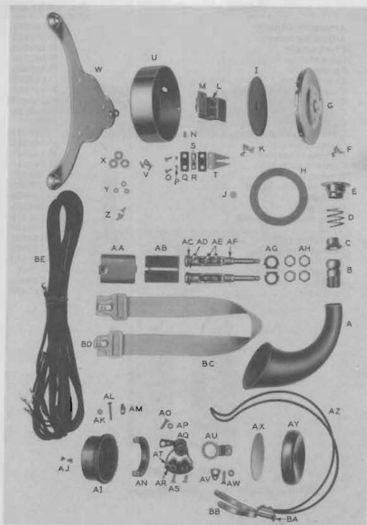
Figure 48—Dispatcher's Head Telephone Set
